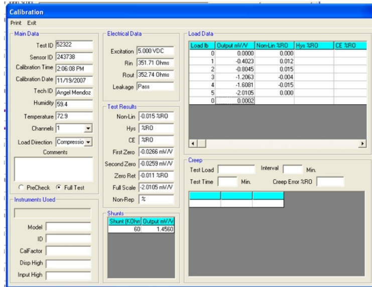
Figure 7, Sensor ID: 243738, LSB200, Calibration results performed on 11/19/2007, before vibration testing, prior to span resistance.
