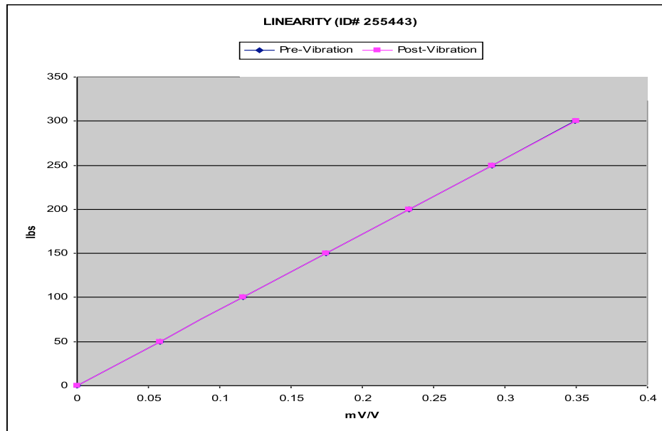
Figure 21, Linearity response curve for ID# 255443.
