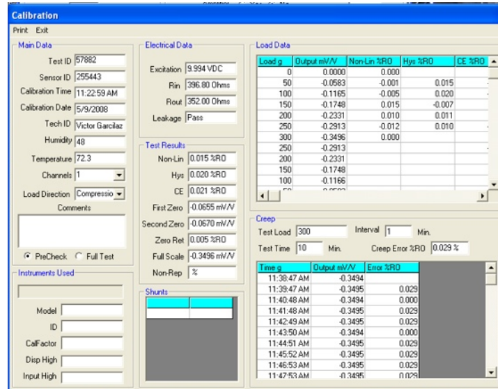
Figure 20, Sensor ID: 255443, LSM400, Calibration results on 4/23/2008, after vibration testing.
