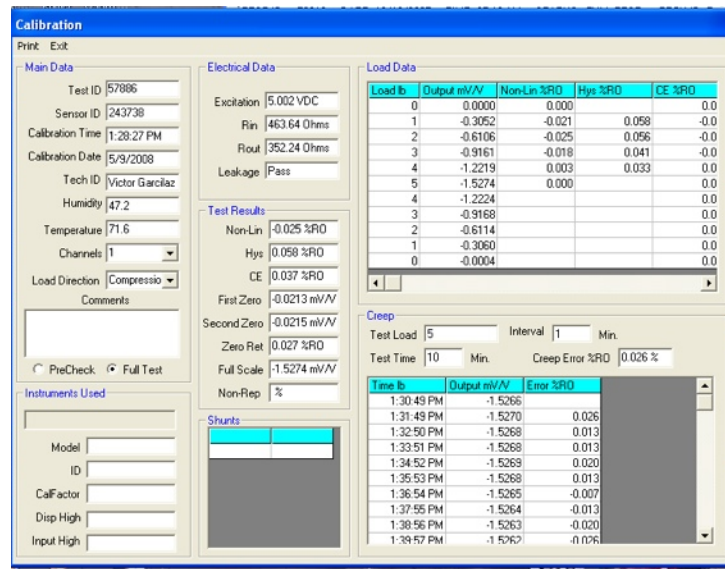
Figure 8, Sensor ID: 243738, LSB200, Calibration results performed on 5/9/2008, after vibration testing, with span resistor.
