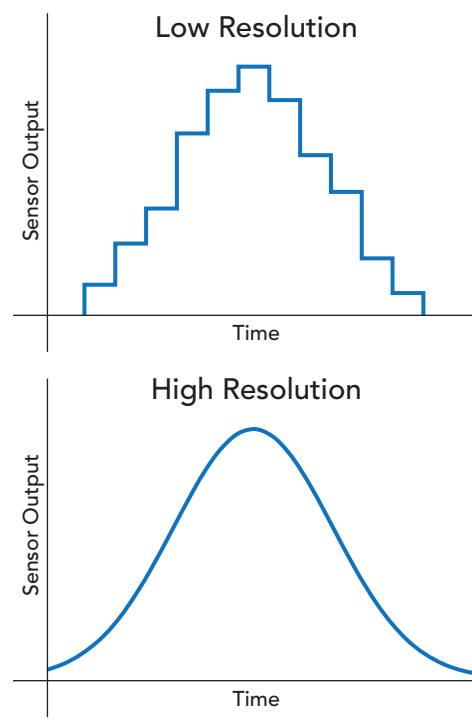
Figure 2: DAQ resolution is the difference between signal measurement and one with steps
